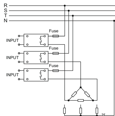
Three Phase Load Application With The Three SSRs
